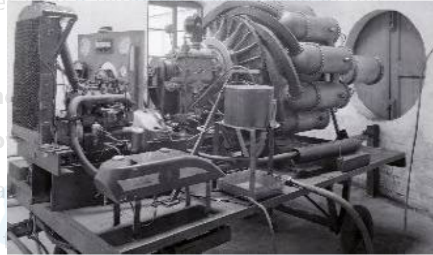
First jet propulsion engine by Frank Whittle, 1938
